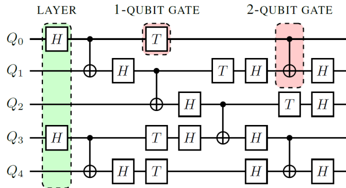
Figure 1: Example of a 5-qubit quantum circuit from [17], with each horizontal line representing the time-evolution of the state of a single logical qubit.
